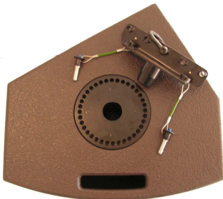
(1) XTLIFTBAR and the I12P enclosure
