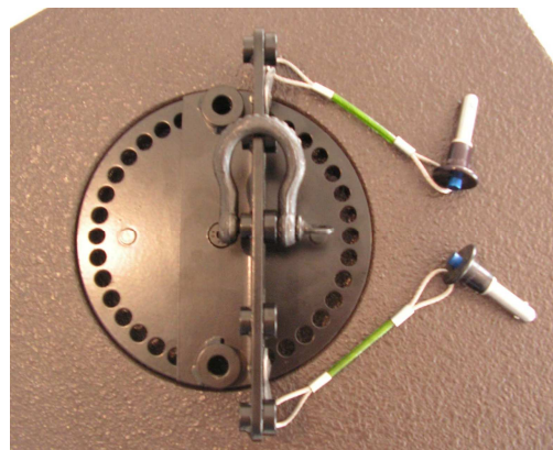
(2) The XTLIFTBAR mounting stud mates with I12P pole mount sockets (top or bottom)
