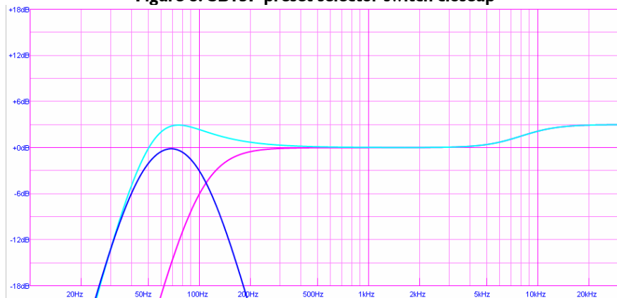
Figure 9: SB15P with positive polarity, 108P or 112P in X-OVER mode provides a 3 dB sub/low frequency contour (rear panel volume at 0 dB)
