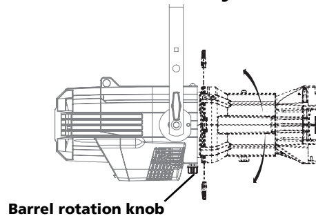
Figure-2.8 Rotating the shutter barrel assembly
