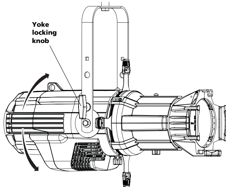
Figure-2.3 Tilting the fixture on the yoke
