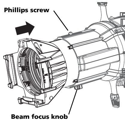
Figure-2.2 Secure lens tube with zoom knob and Phillips screw
