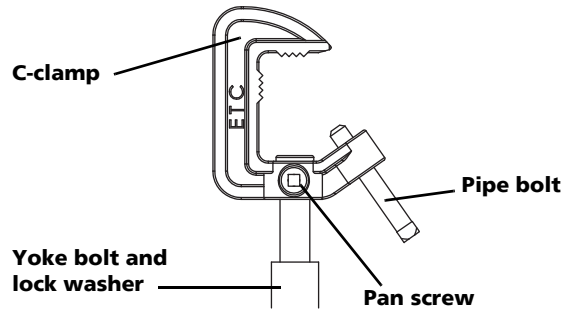
Figure-2.9 Adjusting the c-clamp
