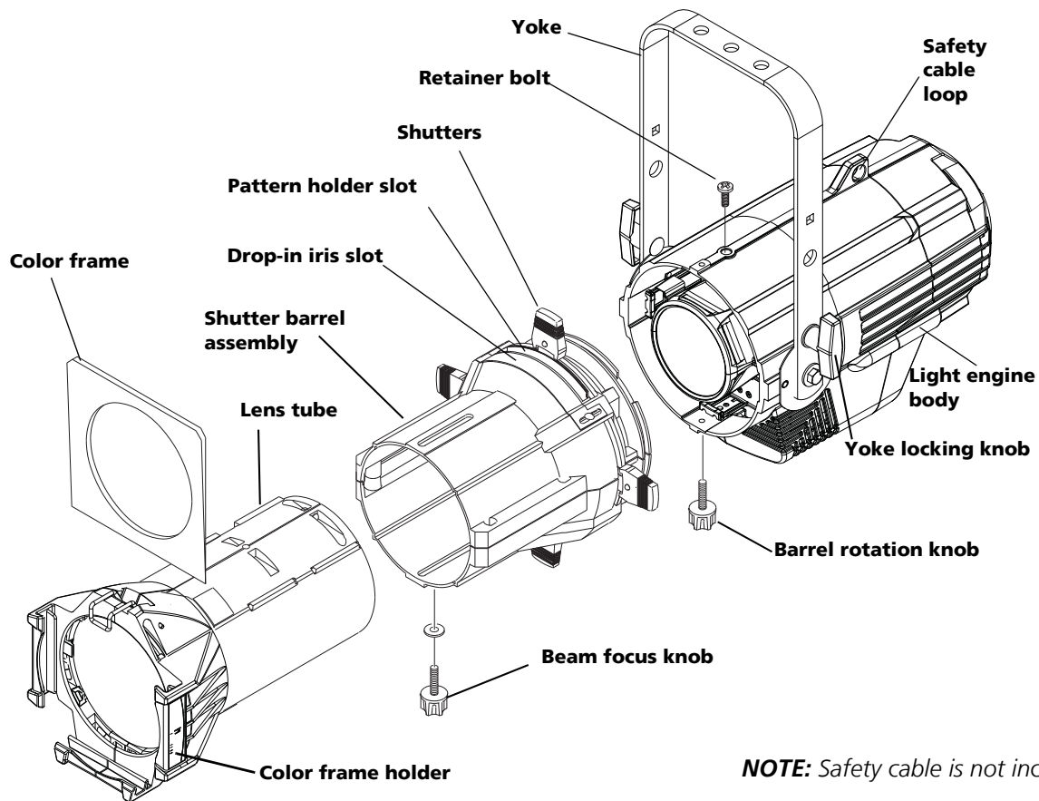
Figure-2.1 Basic assembly
