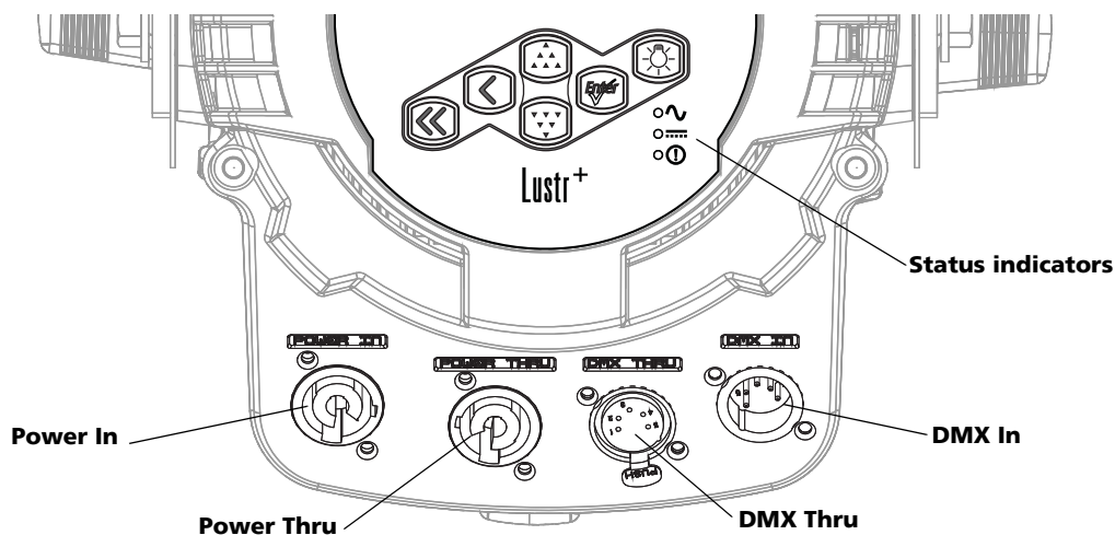
Figure-2.13 Power and DMX connections on back of fixture
