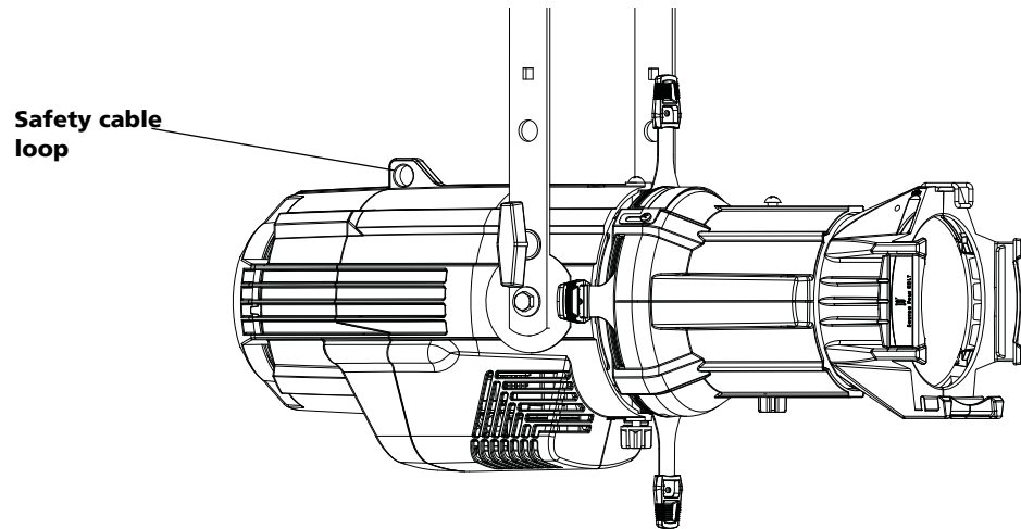
Figure-2.12 Safety cable loop on fixture housing
