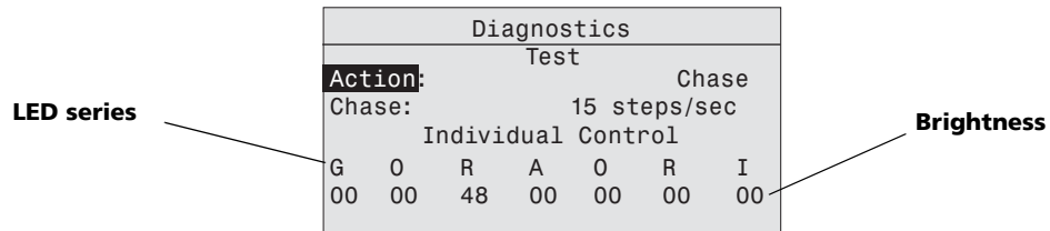
Figure-4.34 Test Screen in Chase mode
